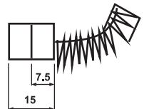
Carbon brush length
